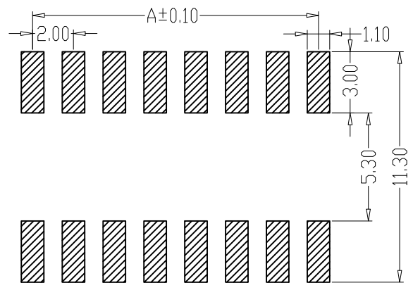
PCB LAYOUT
